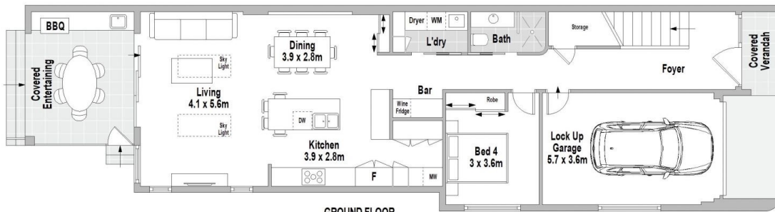
GROUND FLOOR
